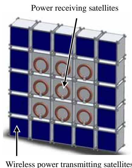
Figure 2 System's conformation before deploying.
