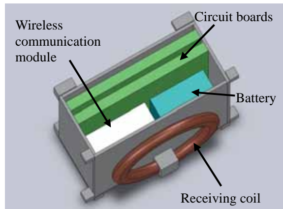
Figure 6 Inner structure of receiving satellite.
