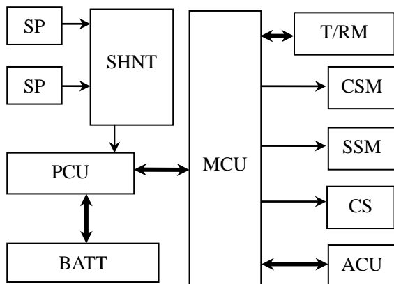
T/RM – Wireless power transmission and receiving module (coils, inflatable).
