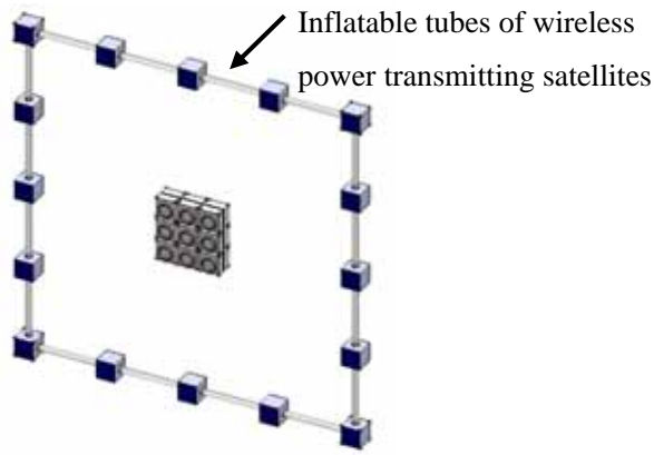
Figure 3 System's conformation after deploying.
