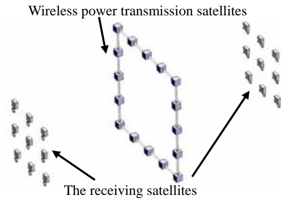
Figure 4 System's conformation after deploying (in regular operation state).
