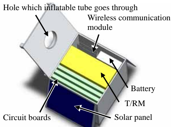
Figure 5 Inner structure of power transmitting satellite.
